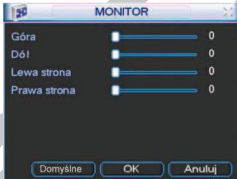
Rys. 5-30. Menu Monitor.
